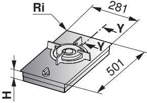
GAS311GKBZ (31073)
