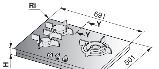
GAS731GKBZ (31075)
